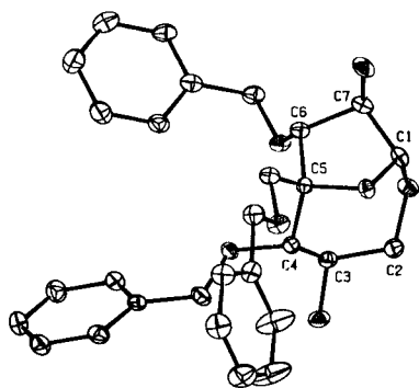
Figure 1. ORTEP drawing of 12
