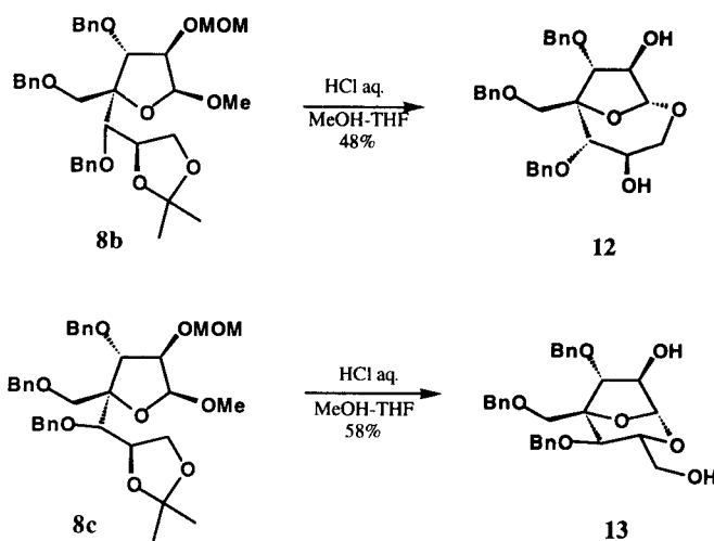
Scheme 6
